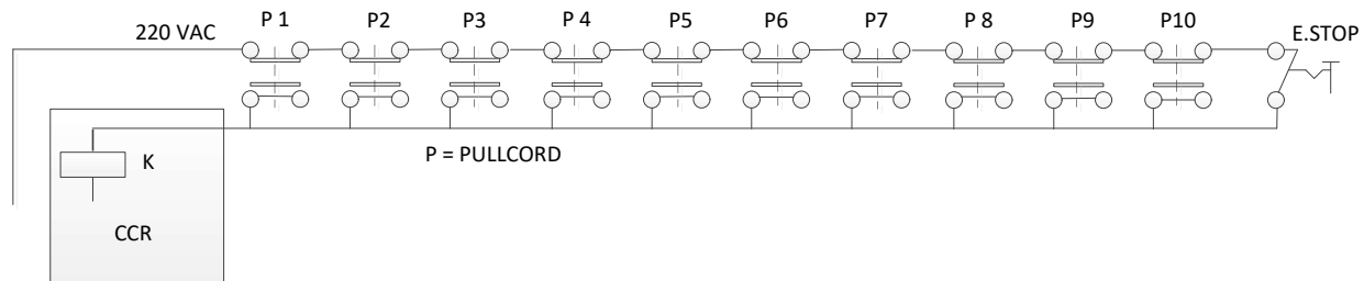
Wiring pullcord 405BC01
